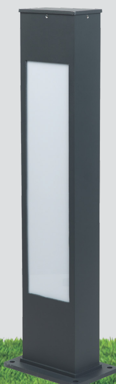
SS 221100 L:8x15 cm H:70 cm Shape/Style : 15w Led : Pleksi Arm. Glass : Aluminium Profile Material : Paint : Electrostatic
